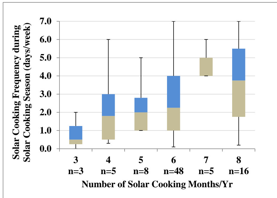
Figure 5: Solar Cooking Frequency (f) as a Function of Climate (S)
